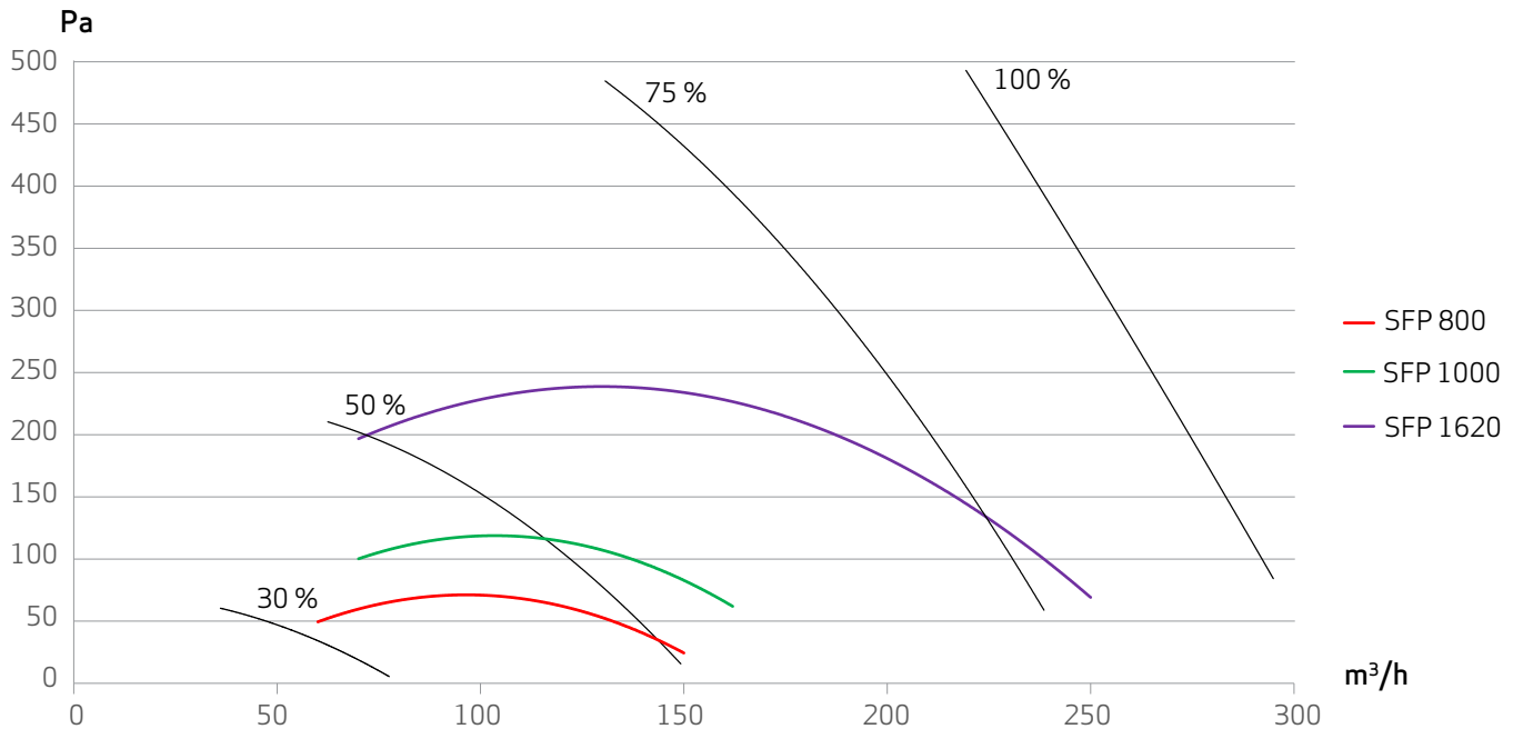
SFP factors ECO 175 - measured according to EN13141-7 (G4/G4 PET)
