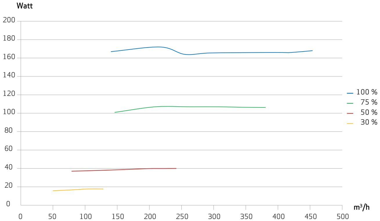
Power consumption
