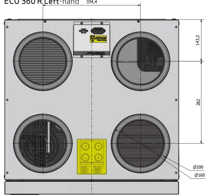
ECO 360 R Left-hand
