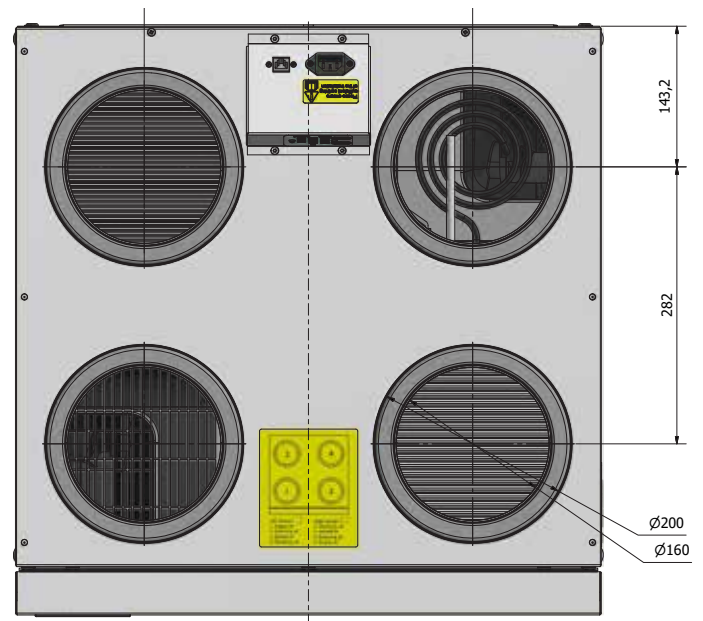
ECO 360 R Right-hand
