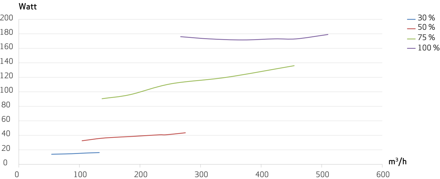
Power consumption
