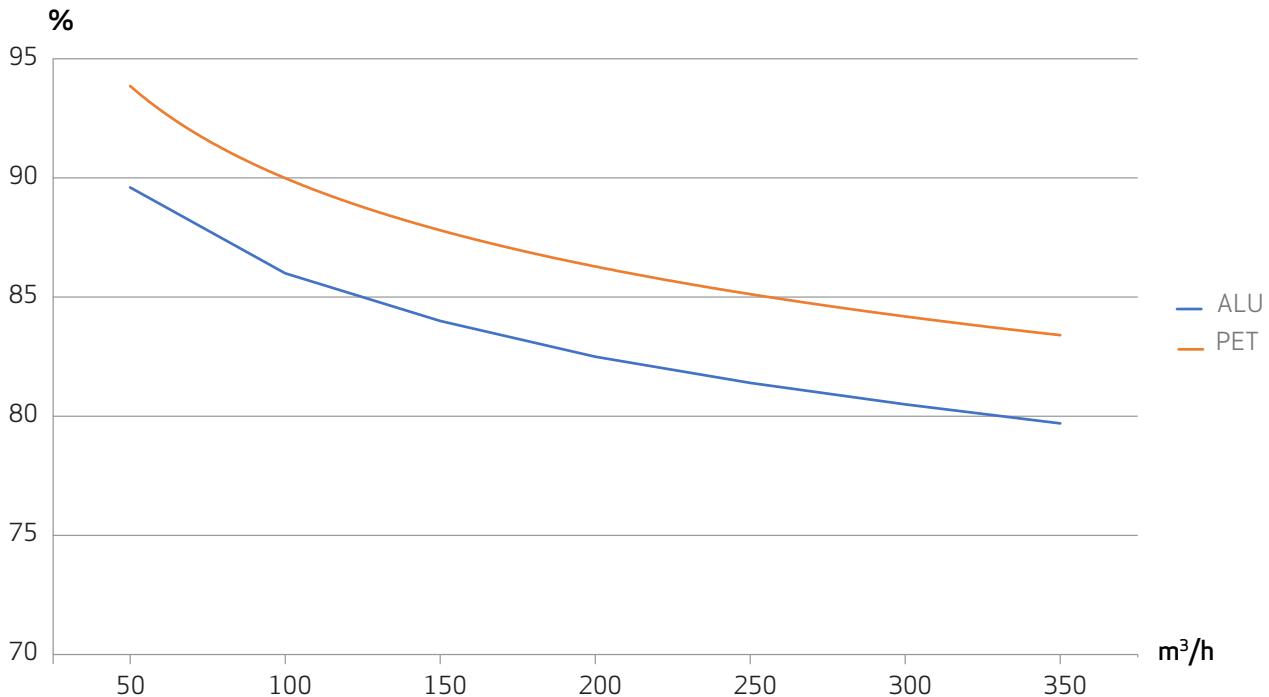
Temperature efficiency according to EN13141-7
