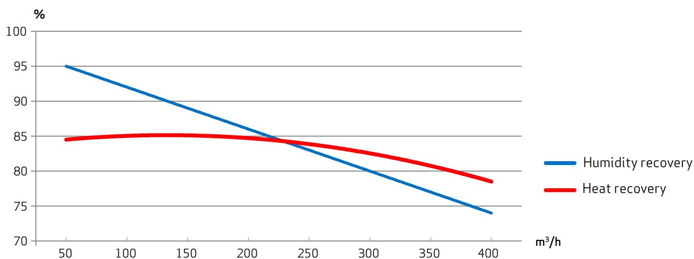
Humidity and temperature efficiency at 25 rpm - measured according to EN 13141-7
